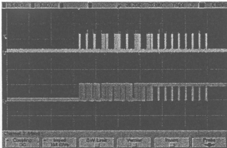
Figure 12: The measured waveforms with four tags
