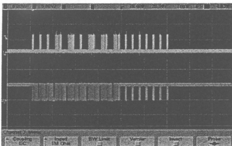
Figure 13: The measured waveforms with five tags
