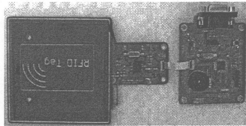
Figure 7: A 13.56 MHz RFID system
