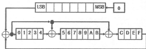
Figure 6: CRC 16/ITU generation scheme
