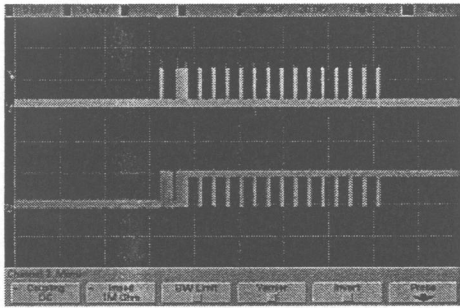
Figure 10: The measured waveforms with a single tag
