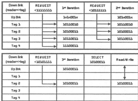
Figure 5: Processing steps for collision-avoidance function
