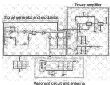
Figure 3: Transmitting block schematic
