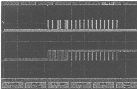
Figure 11: The measured waveforms with two tags
